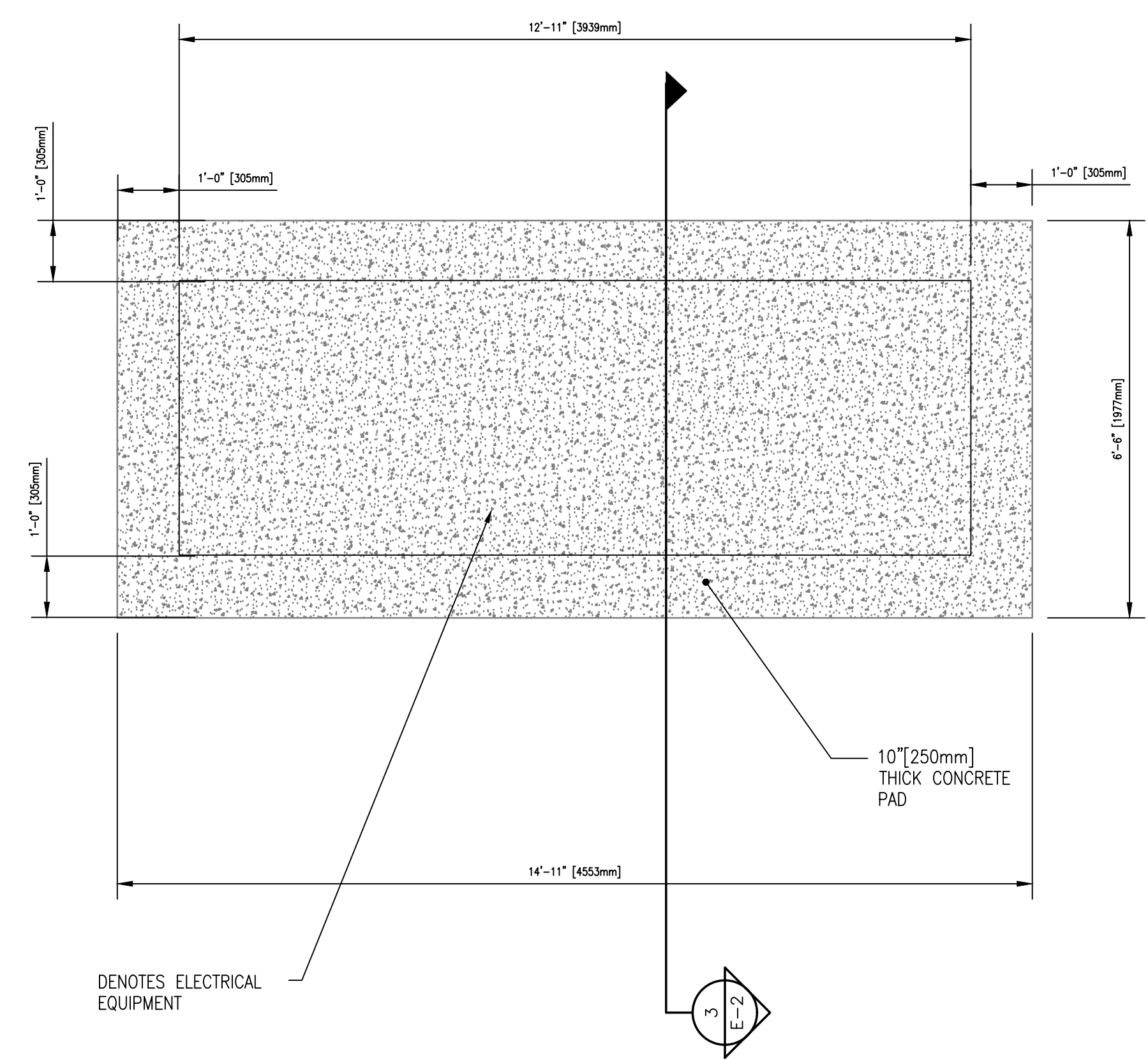
1 CONCRETE SITE PLAN E-2 SCALE: 1/2"=1'-0"
